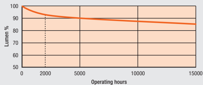
T5 High Efficiency SMARTLUX® Lumen Maintenance
