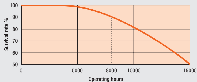
T5 High Efficiency SMARTLUX® Life Expectancy
